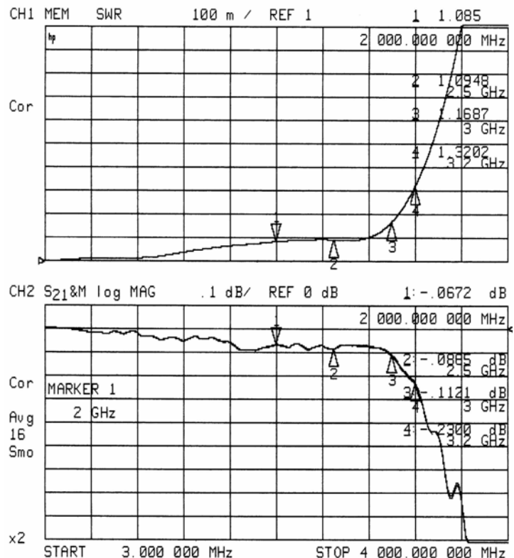
Typical VSWR and Insertion Loss
