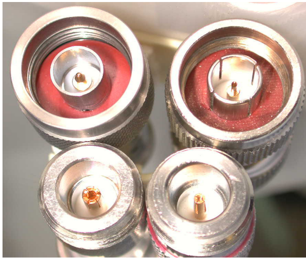
N Connectors Female & Male 50Ω & 75Ω
