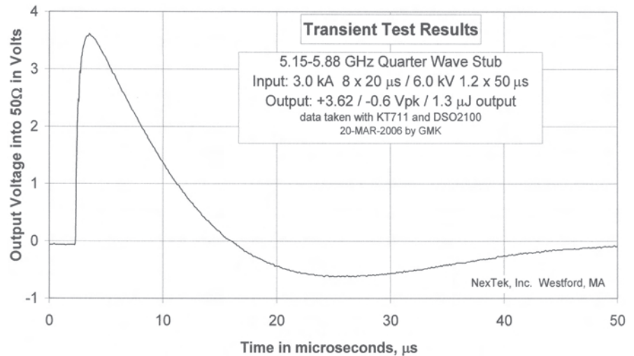
Figure 5. Quarter-wave let-through.
